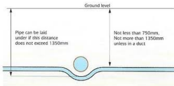
Diagram 6 - Pipes laid under an underground obstruction.
