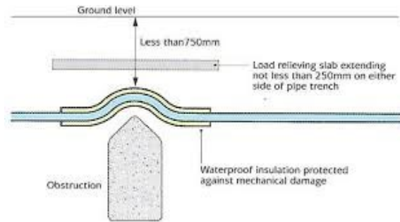
Diagram 5 - Pipes laid shallower than 750mm deep due to an obstruction.
