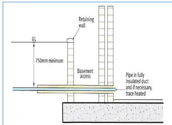
Diagram 7 - Alternative method of supplying water to a building below street level.
